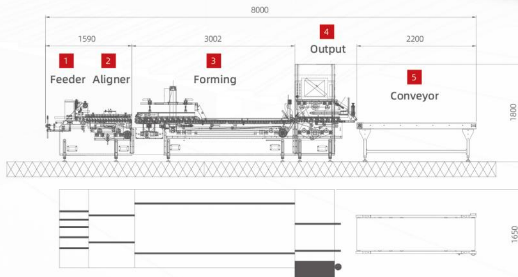
Machine layout
