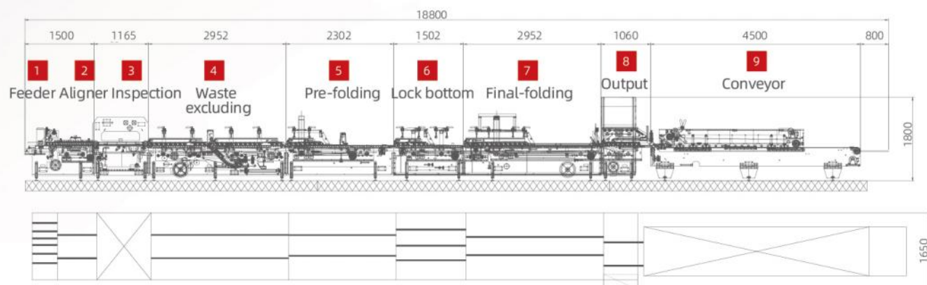
Machine layout
