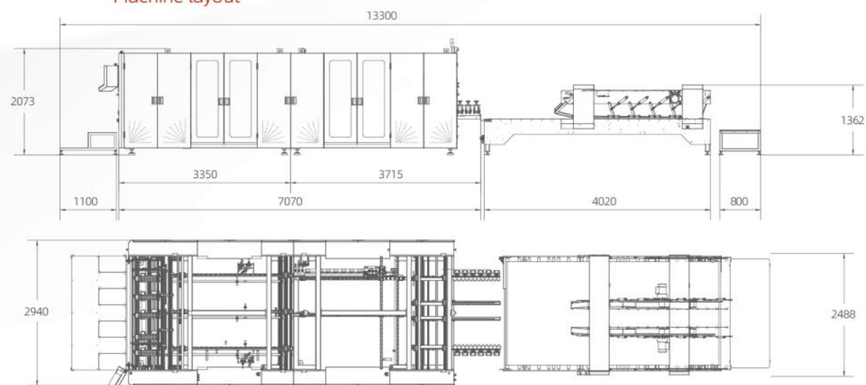
Machine layout
